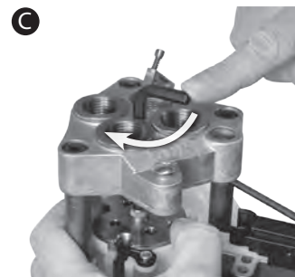
Raise carrier to the mid-stroke position, install shell plate, lightly tighten clockwise with 1/4" hex head wrench.
