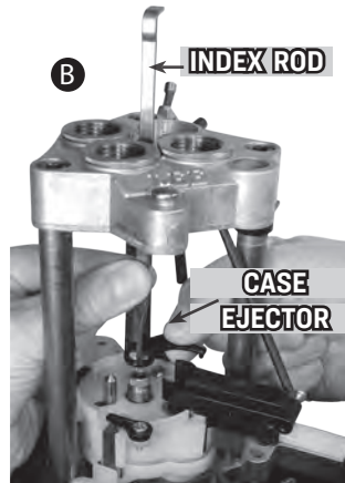
Remove index rod and case ejector.
