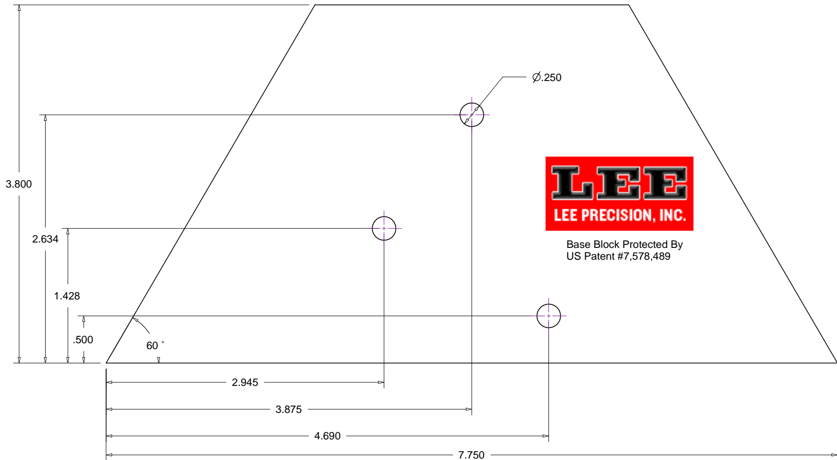
Lee Breech Lock Challenger Press Mounting Hole Layout
